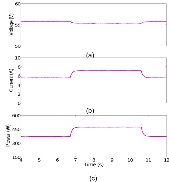
Hardware test- DG#1 performance during load change: a) Dc link voltage, b) dc-dc converter inductor current, and c) DG output power
