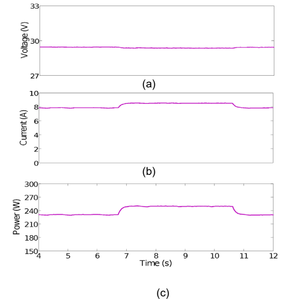
DG#2 performance during load change: a) Voltage at dc link, b) dc-dc converter inductor current, and c) DG output power
