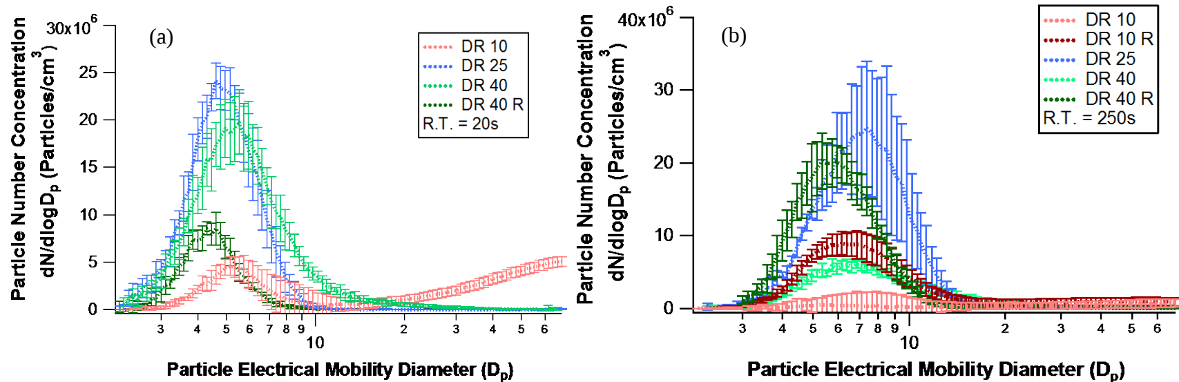
Figure 3-19: Particle Size Distributions at a Fixed Residence Time (a) R.T. = 20s (b) R.T. = 250s
