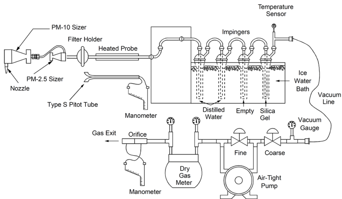
Figure 1-3: EPA Method 201A Sampling Train
