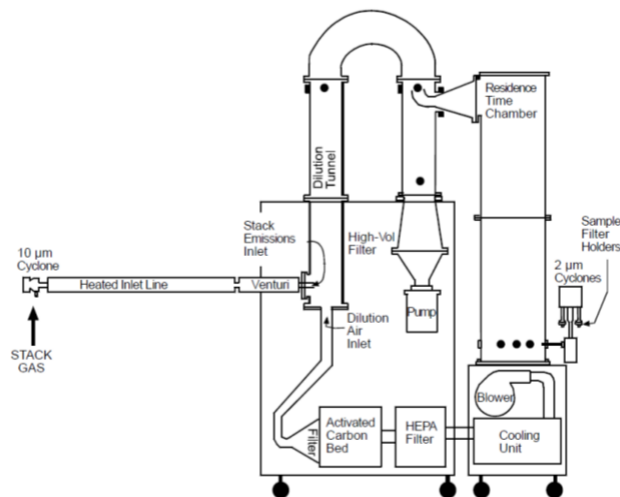
Figure 1-6: Hildemann Dilution Design
