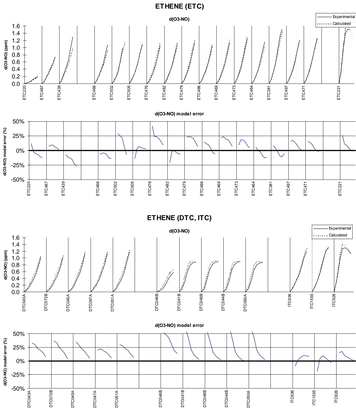
Figure 21. Results of model simulations of d(O_3-NO) in the ethene - NO_x experiment carried out in the blacklight chambers. Runs are ordered by ROG/NO_x except for the 13 replicate ETC experiments (middle of top plot), which are ordered by temperature.
