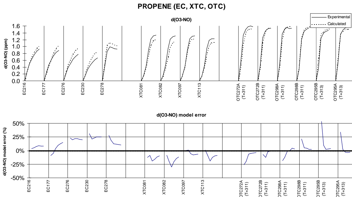
Figure 25. Results of model simulations of d(\text{O}_3\text{-NO}) in the propene - \text{NO}_x experiment carried out in the xenon arc or outdoor chambers. Runs are ordered by \text{ROG}/\text{NO}_x .
