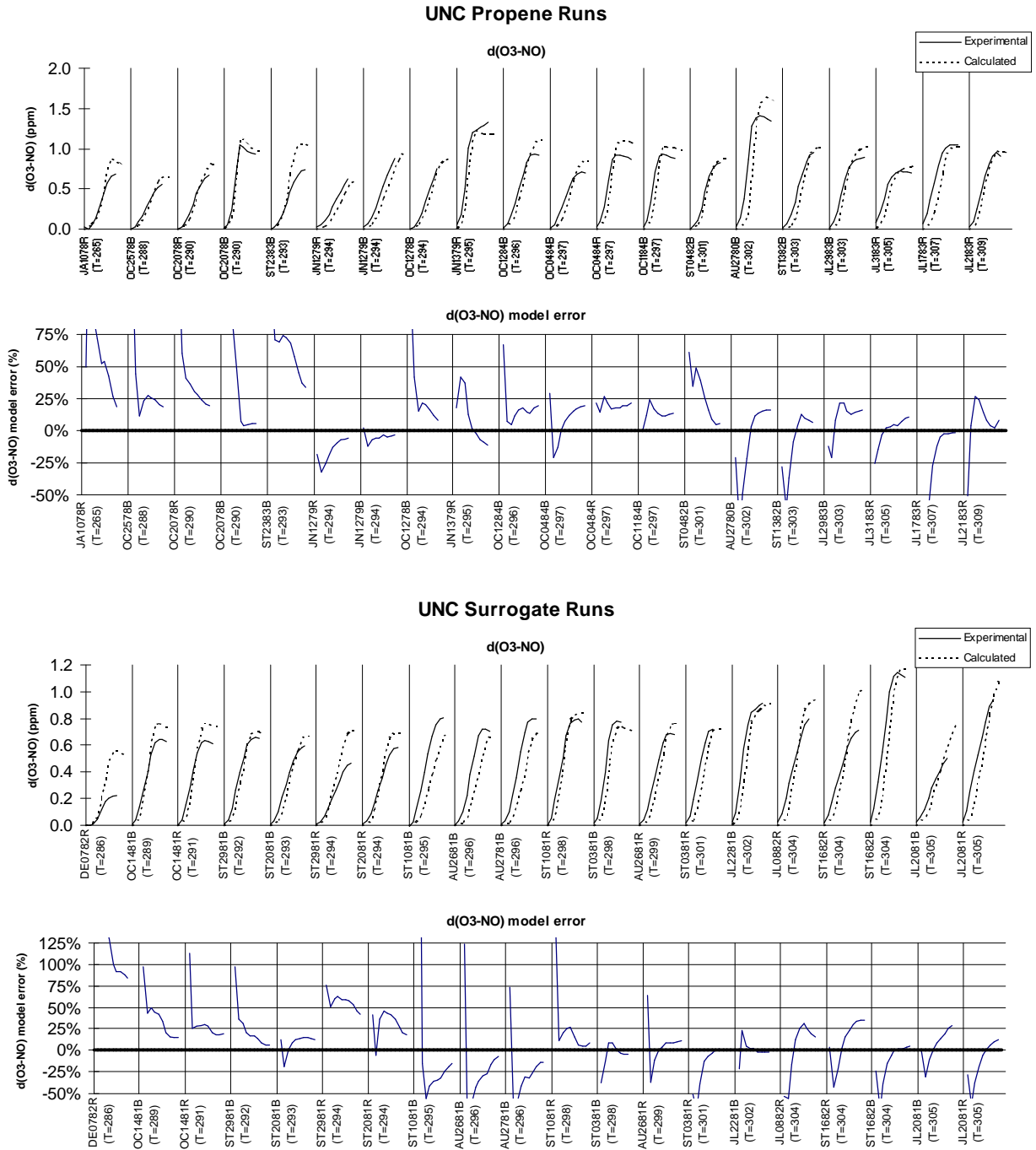
Figure 35. Results of model simulations of d(O 3 -NO) in propene - NO x and surrogate - NO x experiments carried out in the UNC outdoor chamber. Runs are ordered by temperature.
