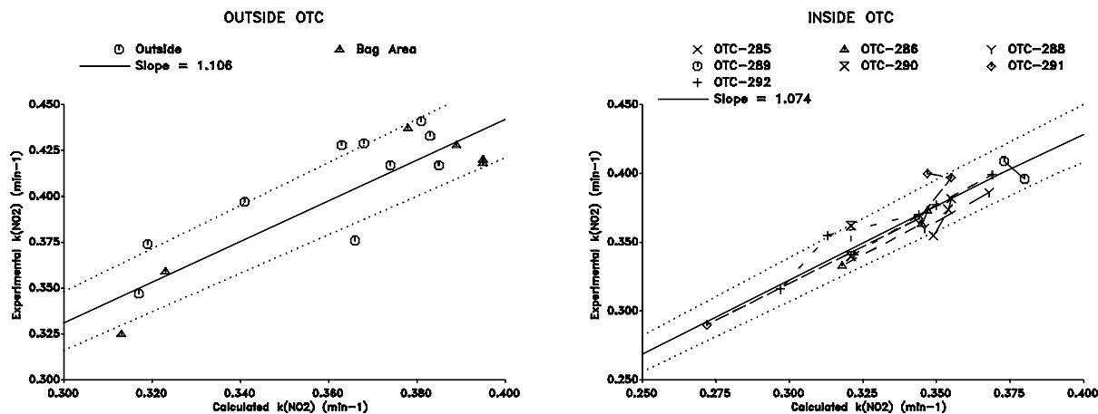
Figure 12. Plots of experimental vs calculated NO 2 photolysis rates measured in or around the Outside Teflon Chamber.
