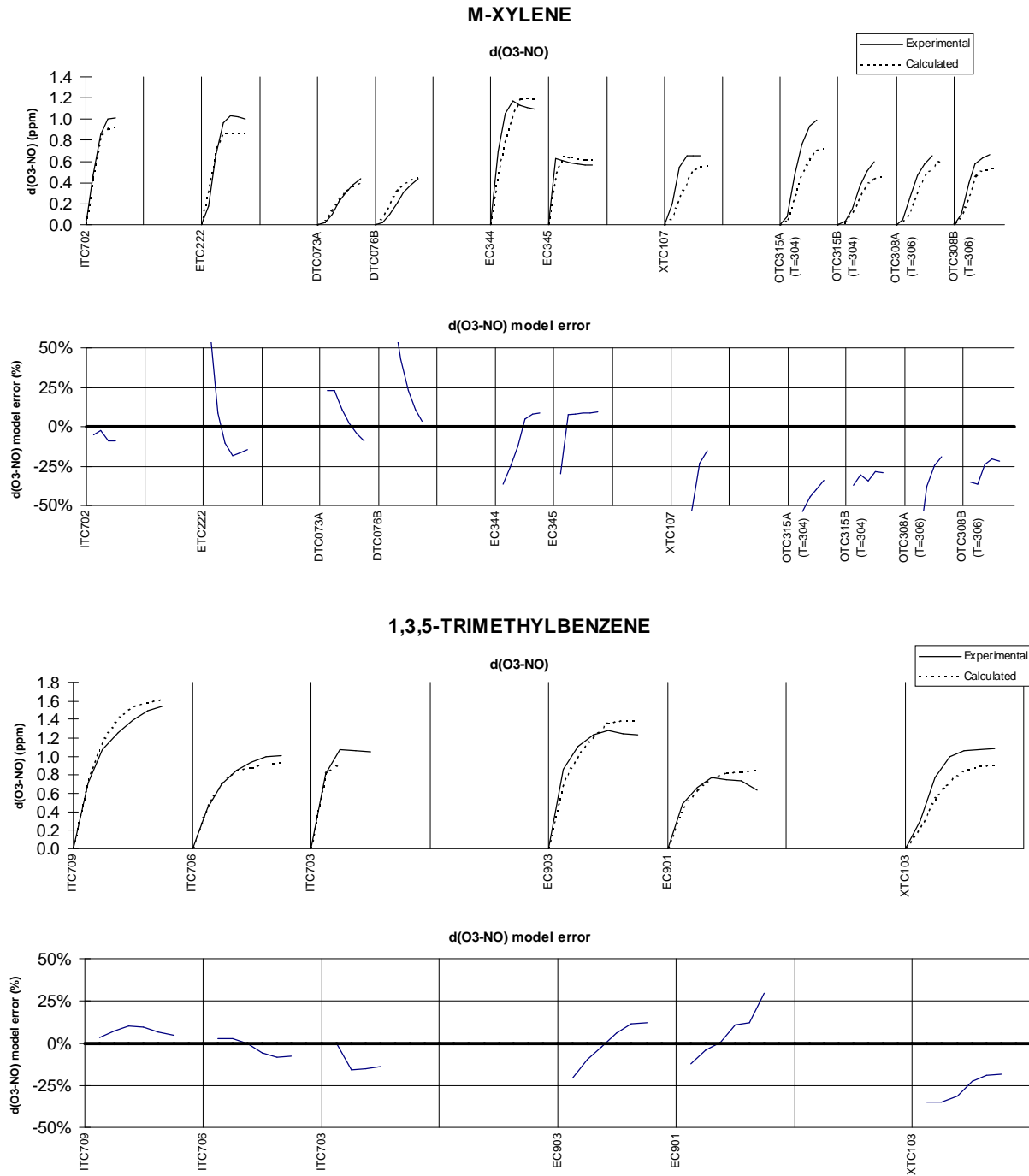
Figure 29. Results of model simulations of d(O 3 -NO) in the m-xylene - NO x and 1,3,5-trimethylbenzene - NO x experiments. Runs are ordered by ROG/NO x .
