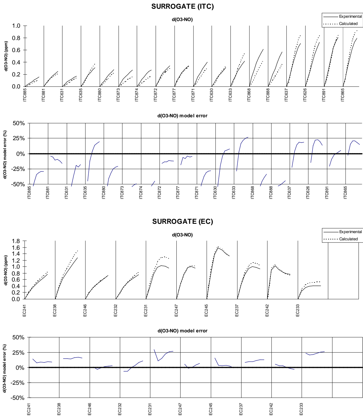
Figure 32. Results of model simulations of d(\text{O}_3\text{-NO}) in surrogate - \text{NO}_x experiments carried out in the ITC and the EC. Runs are ordered by \text{ROG}/\text{NO}_x .
