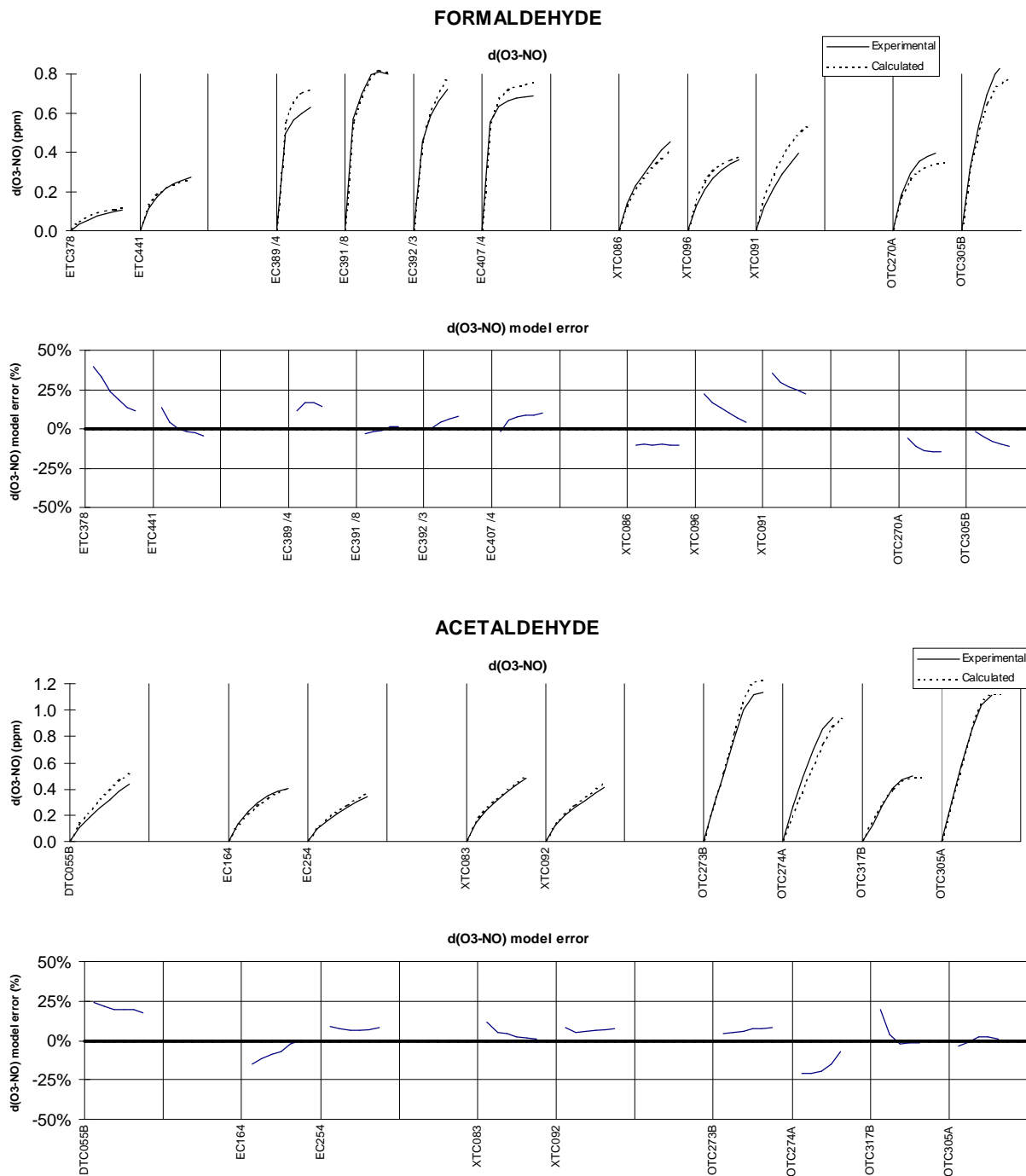
Figure 20. Results of model simulations of d(O 3 -NO) in the formaldehyde - NO x and the acetaldehyde - NO x experiments.
