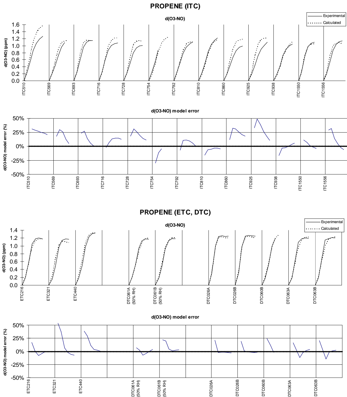
Figure 24. Results of model simulations of d(O 3 -NO) in the propene - NO x experiments carried out in the blacklight chambers. Runs are ordered by experiment number.
