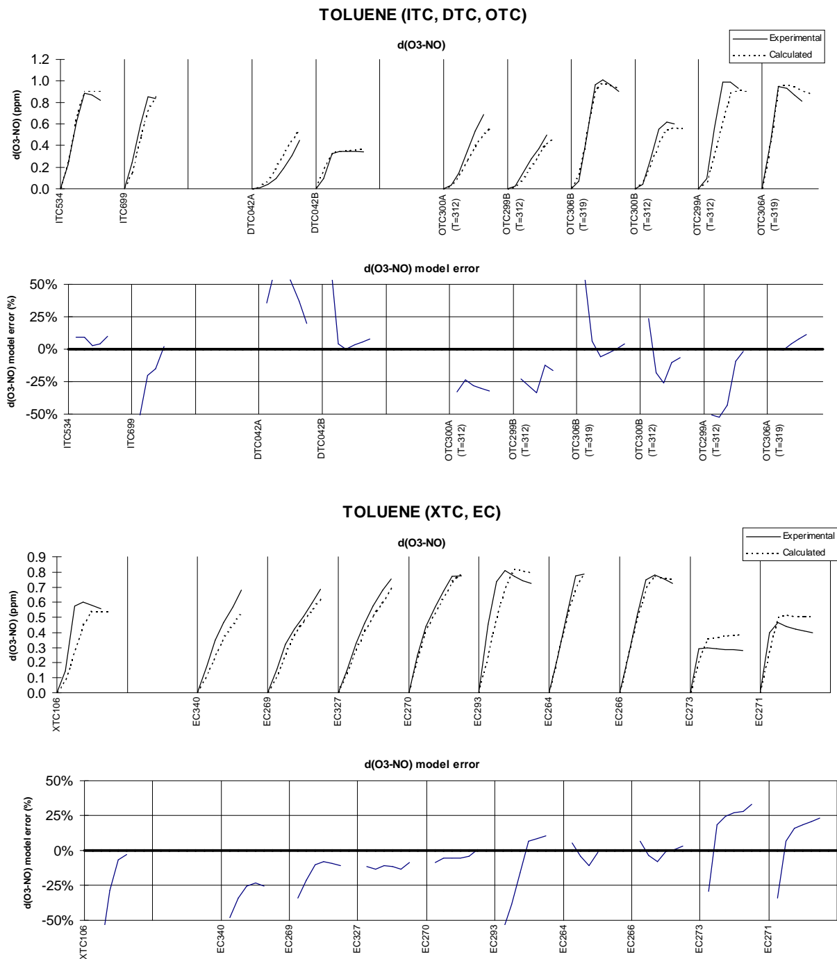
Figure 27. Results of model simulations of d(\text{O}_3\text{-NO}) in the toluene - \text{NO}_x experiments. Runs are ordered by \text{ROG}/\text{NO}_x .
