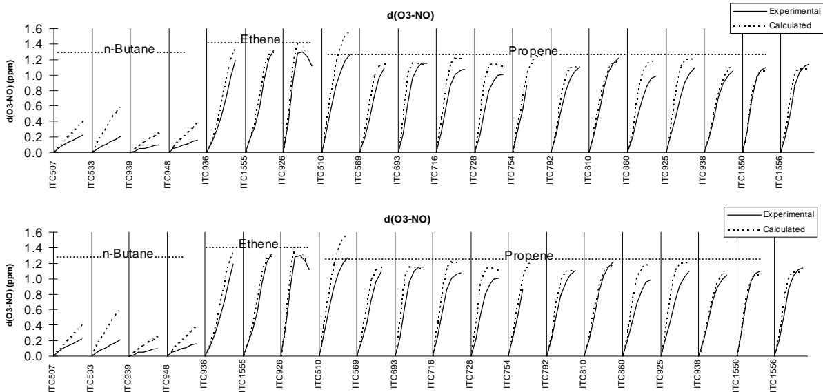
Figure 13. Results of model simulations of d(O_3-NO) of the n-butane - NO_x , ethene - NO_x and propene - NO_x experiments carried out in the SAPRC ITC, where the model used the radical source assignments used in the SAPRC-90 and RADM-2 mechanism evaluations. "Model error" is normalized bias (see text).
