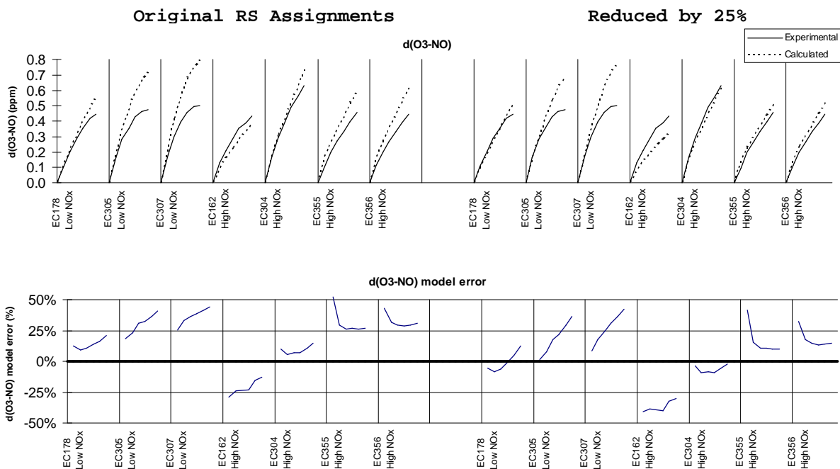
Figure 16. Results of model simulations of d(\text{O}_3\text{-NO}) in the EC n-butane - \text{NO}_x runs using the previous and the adjusted radical source assignments.
