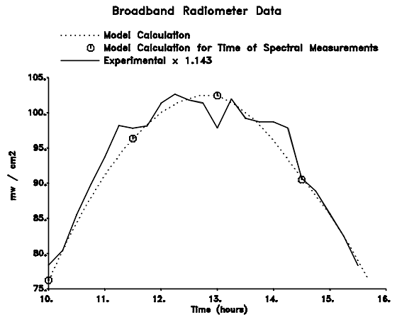
Figure 7. Examples of fits of adjusted solar light model to light characterization data for two outdoor chamber runs. Top plots: fits to direct and diffuse spectral data. Bottom plots: fits to changes with time in the data from the UV and broadband radiometers.
