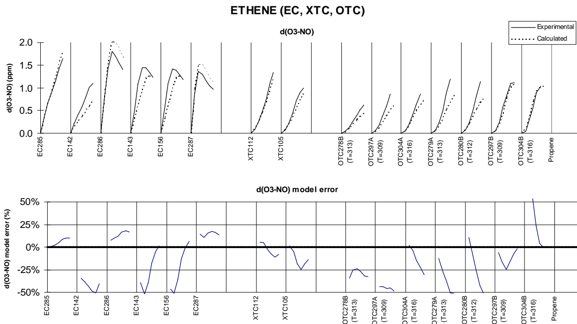
Figure 22. Results of model simulations of d(\text{O}_3\text{-NO}) in the ethene - \text{NO}_x experiment carried out in the xenon arc or outdoor chambers.
