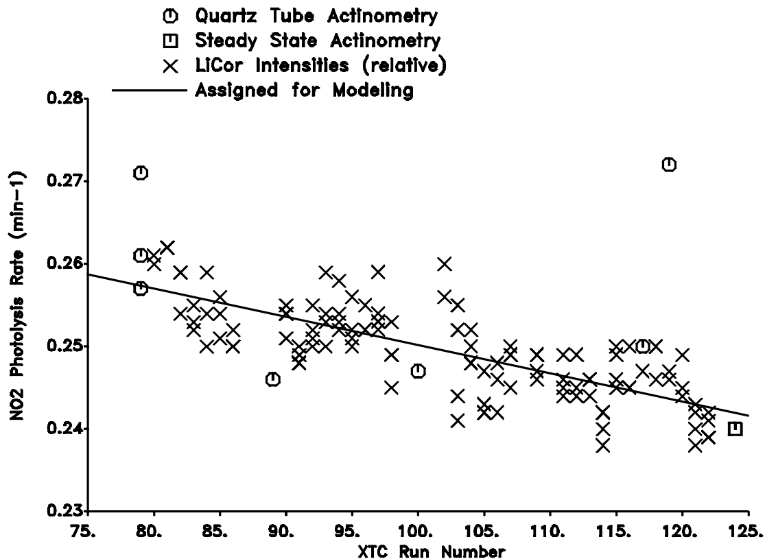
Figure 8. Plots of NO 2 photolysis rates in the XTC chamber against XTC run number.
