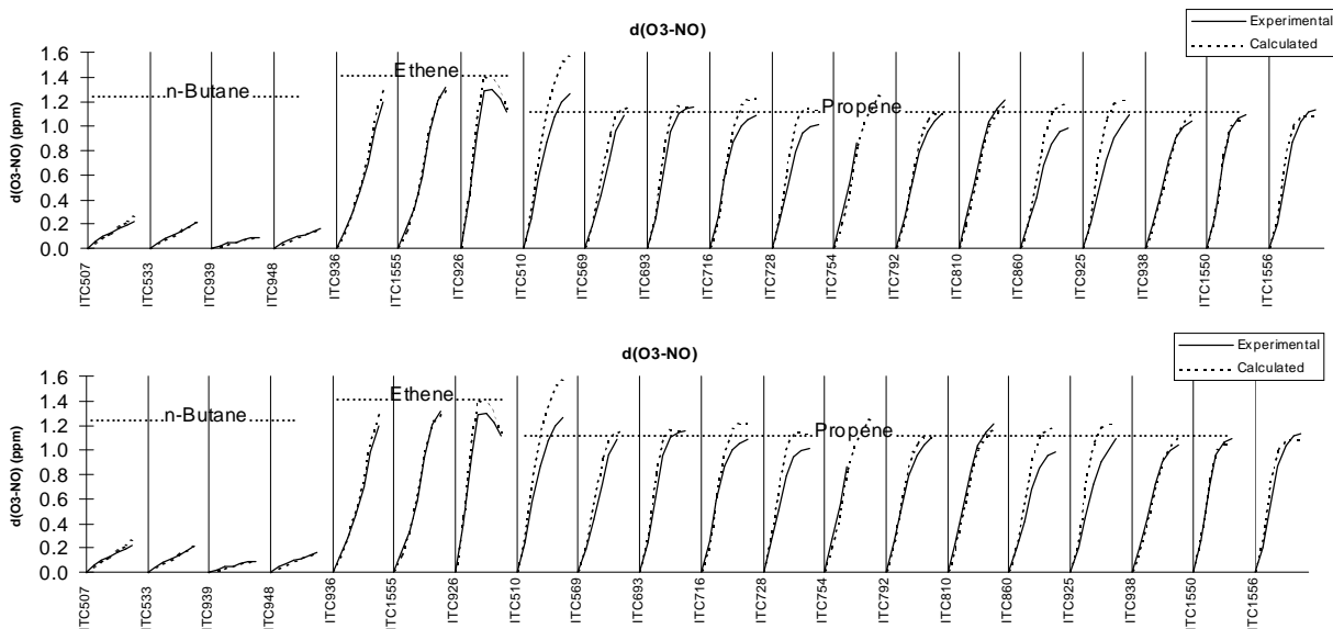
Figure 14. Results of model simulations of d(O_3-NO) of the n-butane - NO_x , ethene - NO_x and propene - NO_x experiments carried out in the SAPRC ITC, where the model used the radical source assignments adjusted to fit the n-butane runs. Figure 16. Results of model simulations of d(O_3-NO) in the EC n-butane - NO_x runs using the previous and the adjusted radical source assignments.
